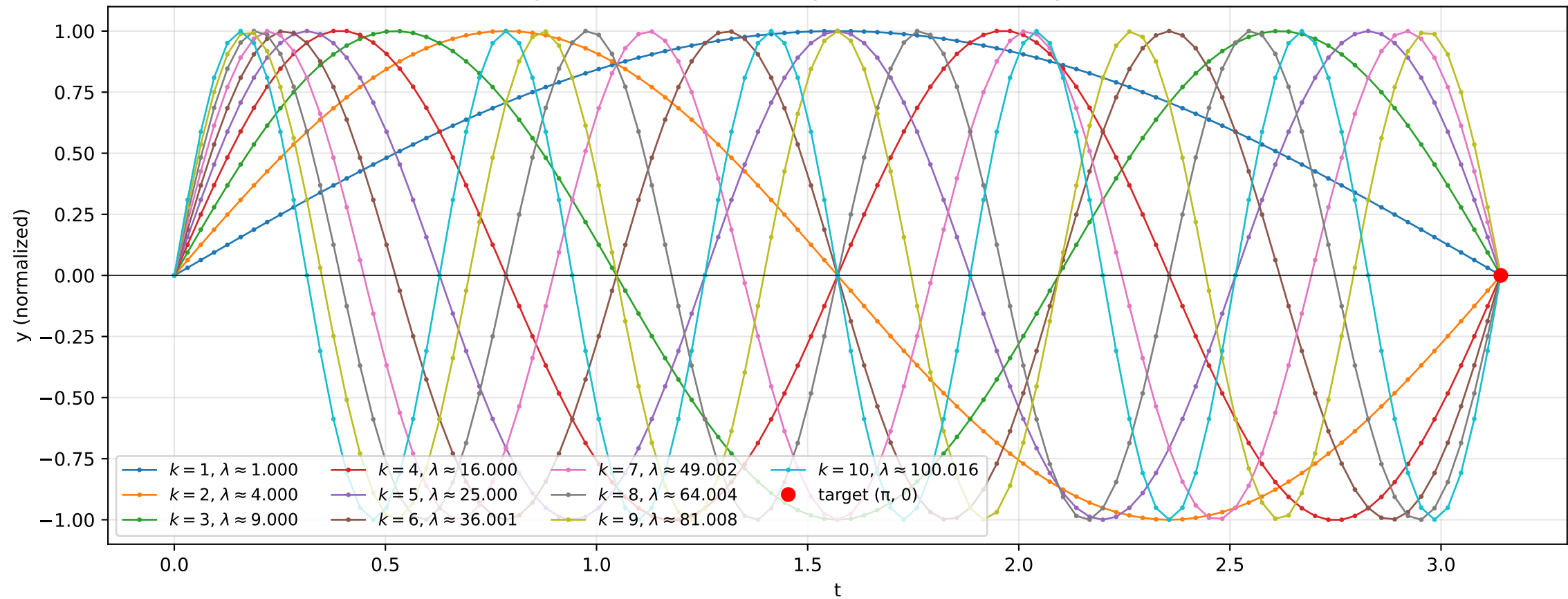
Eigenfunctions on uniform grid (n=100) for 10 eigenvalues
